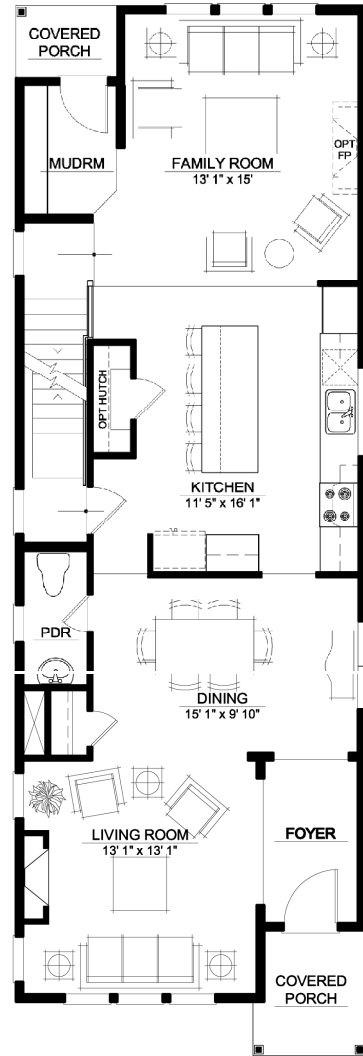
Main floor
